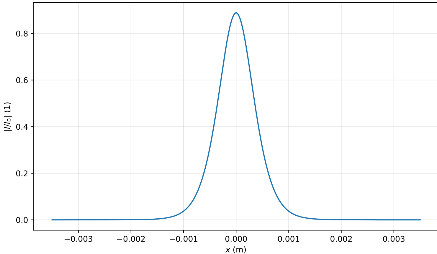
Intensity profile I(x, y = 0, z = 3.901m)/I_0 , P_{in}=0.8P_{cr} , artificial time
